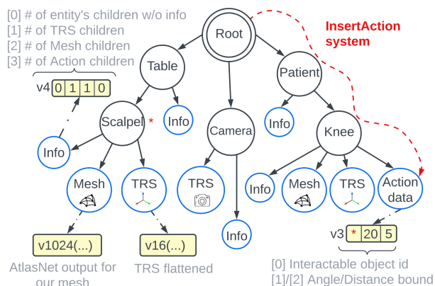
Figure 2. An example of the UniSG. Black nodes represent entities of the ECS architecture, whereas blue nodes are components (e.g., transformations, meshes, actions, etc.), that encapsulate data. Systems (red lines) digest components’ data and perform specified tasks, while traversing the graph. In this case, the InsertAction system checks if the scalpel’s placement on the knee is within the specified spatial bounds, when visiting the ActionData component. Graph features, in yellow, are provided in vector form, digestible by GNNs.
