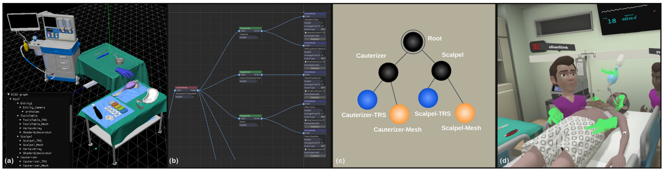
Figure 1. The proposed universal scenegraph unifies (a) the 3D scenegraph with Entity-Component-Systems, (b) the behavioral learning scenegraph, and (c) the deriving GNN graph, towards (d) generative AI for a VR training session.
