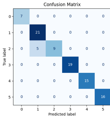
Figure 2: The confusion matrix of the convolutional neural network for the 6 classes.
