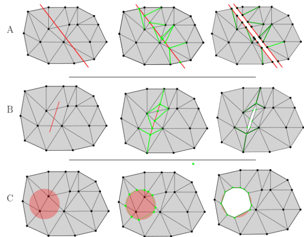
Figure 2: Performing (A) Cut, (B) Tear and (C) Drill on a triangular mesh. The red line represents a plane in (A) and (B). For the Drill case, we simply project the 3D-mesh to a plane and therefore reduce the face versus drill predicate to a simpler 2D-triangle versus circle.
