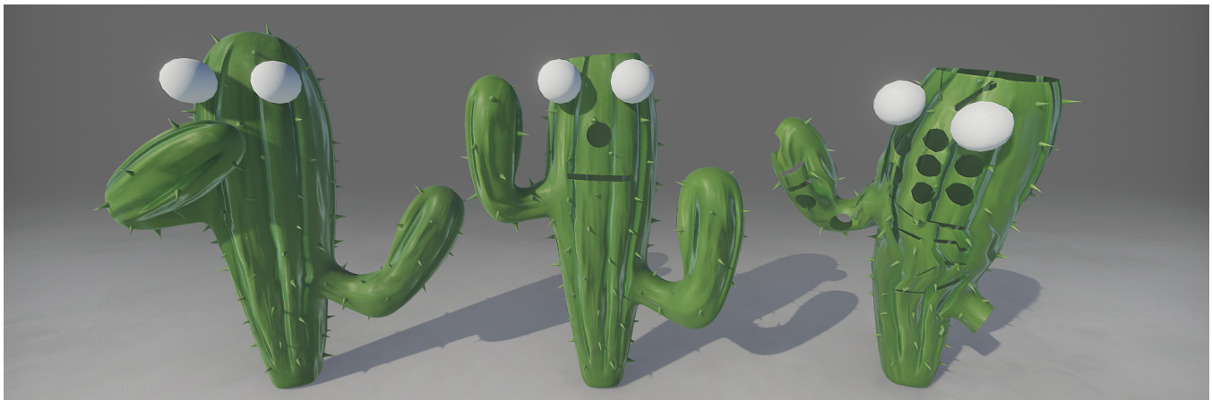
Figure 1: A linear-blend skinned 3D model (left), current state-of-the-art of predefined cut, tear and drill (center), our ‘deep-cut’ framework for unconstrained, arbitrary cuts, tears, drills with soft-body deformations in mobile VR (right)
